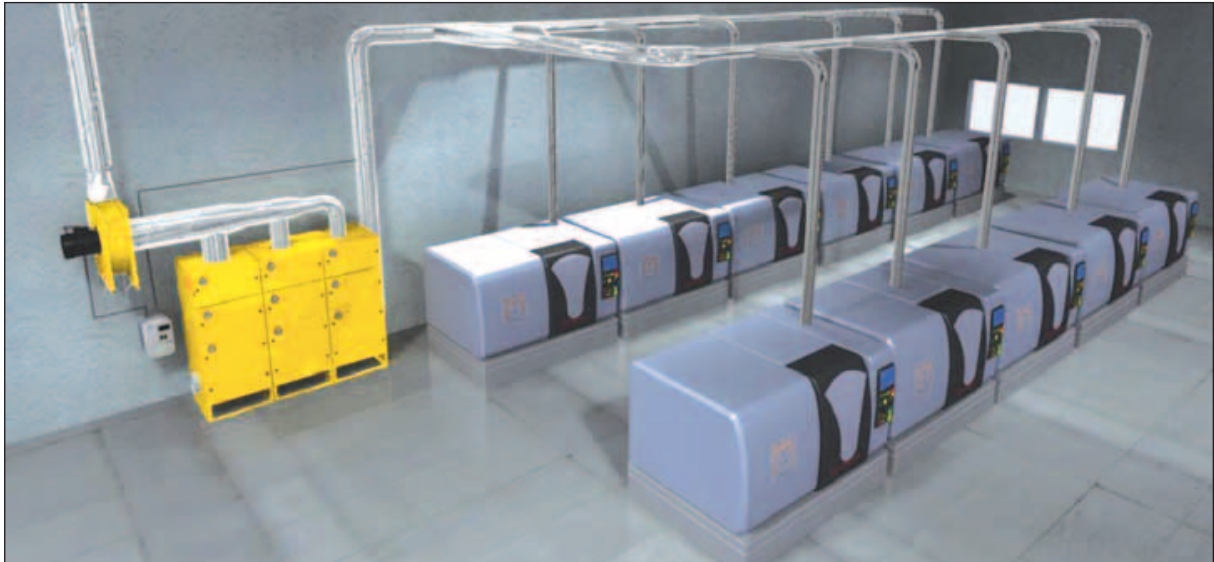
MistEliminator connected to central fan in machine hall
